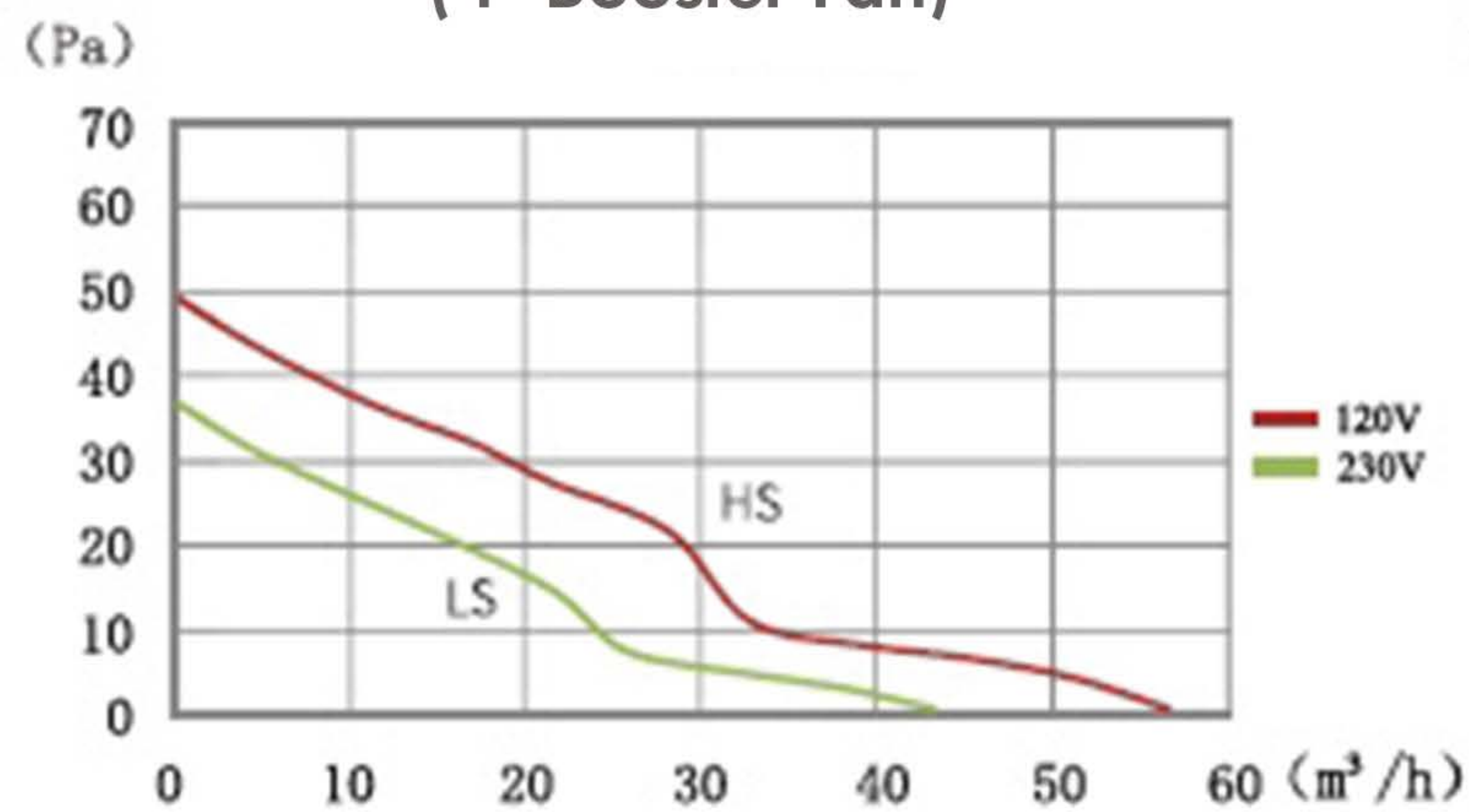
HI-100IS (4" Booster Fan)
